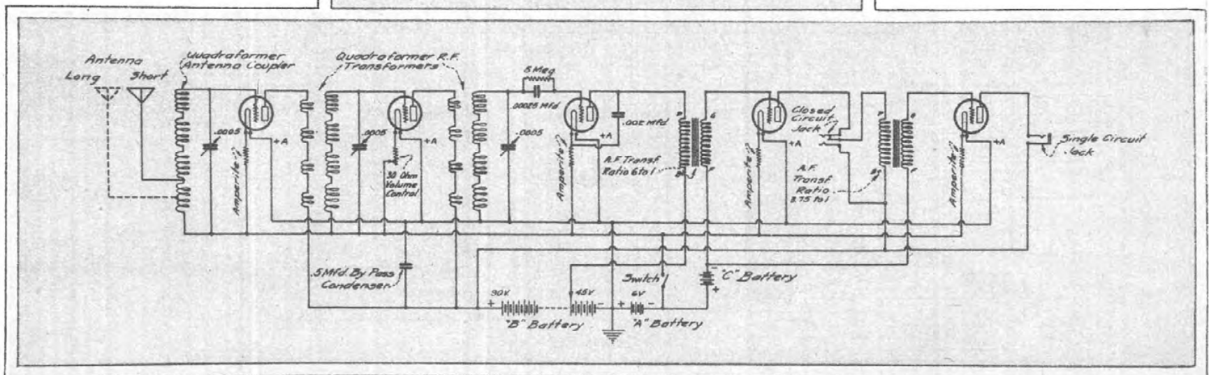
Fig. 2. Wiring diagram of the Quadraformer receiver
