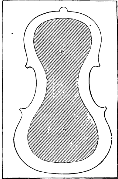
FIG. 78.—Plank for tracing the outline of a fiddle.
