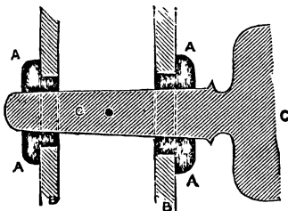
FIG. 98.—Patent Peg to ensure Firmness.
