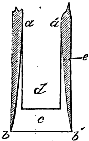
Fig. 194.—Base of peg-box prepared to splice on to neck.
