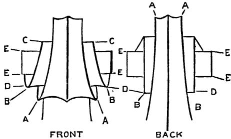
FIG. 165.—Front and back of Volute (Geometrical).
