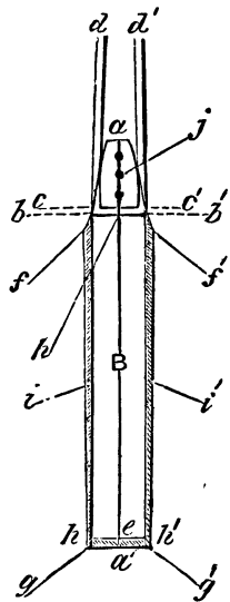
FIG. 196.—Operation of splicing head on to neck.
