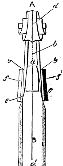
Fig. 193.—Operation of splicing head on to neck (front view).
