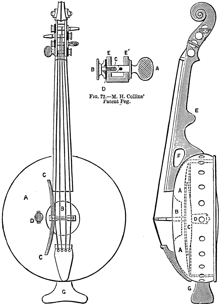
FIG. 71.—M. H. Collins' "Echolin" in plan and section.
