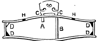
FIG. 83.—Section of the Violin across the ff holes.
