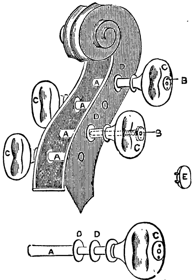
FIG. 97.—Wallis's Patent Peg.
